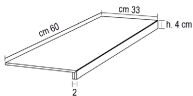
Step Tread 60x33cm
